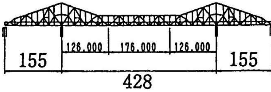
LSB40108,BAY,
