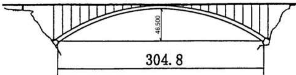
LSB30115,LEWISTON-QUEENSTON,
