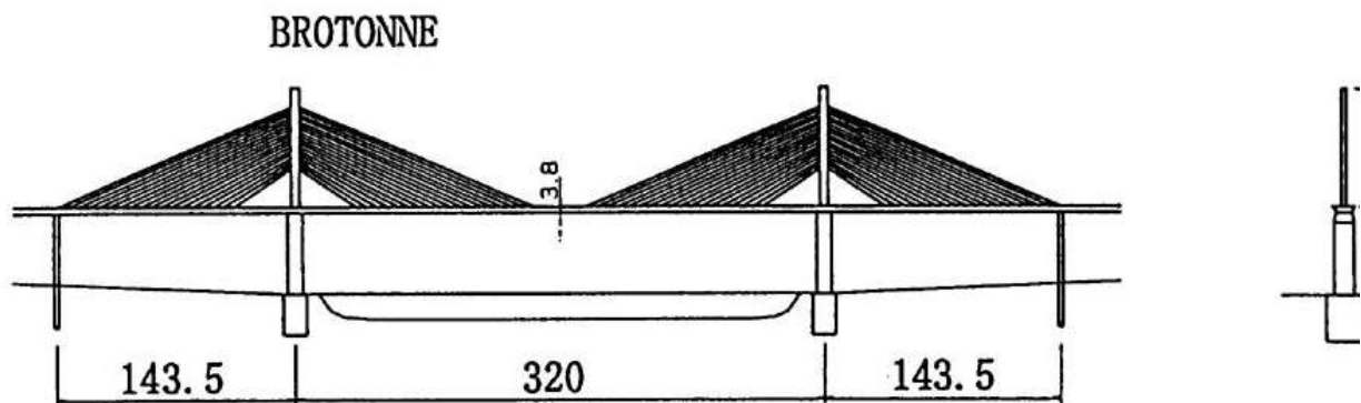
LSB20215,INTERNATIONAL GUADIANA,
