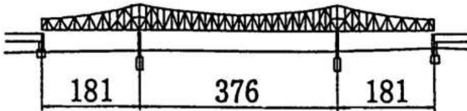
LSB40109,BATON ROUGE,
