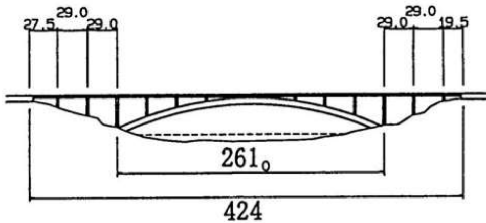
LSB30207,RANCE,
