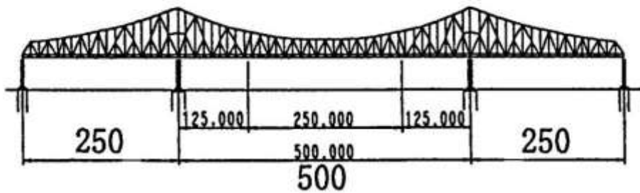
LSB40104,COMMODORE-JOHN-J-BARRY,
