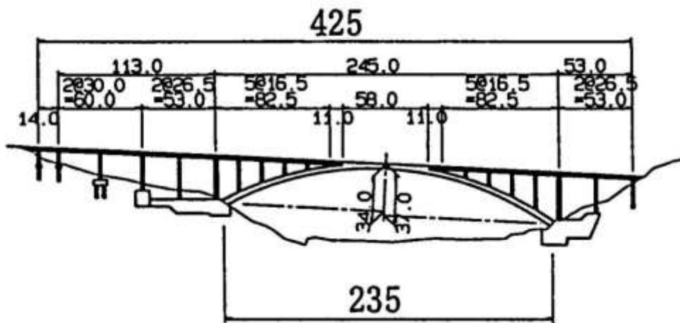
LSB30210, BEPPU-MYOBAN, 別府明礬橋
