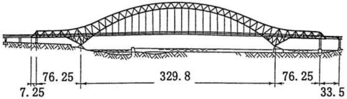
LSB30110,RUNCORN-WINDEZ,
