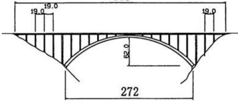
LSB30204,BLOUKRANS,
