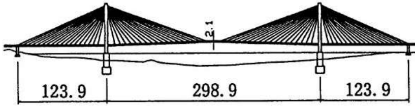
LSB20217,INTER-CITY (PASCO-KENNEWICK),
