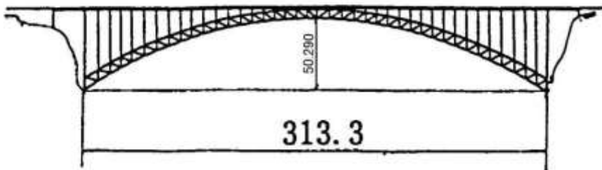
LSB30113,GLEN-CANYON,
