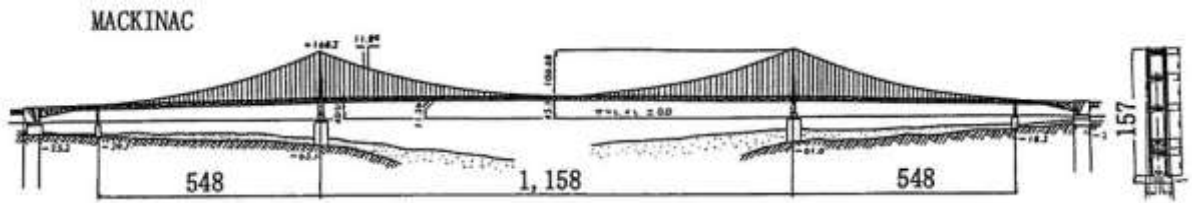
LSB10109, MACKINAC,
