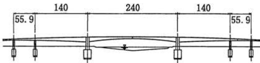
LSB50306,HAMANA,浜名大橋,
