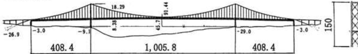
LSB10117,FORTH ROAD,
