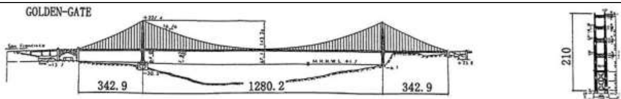
LSB10107, GOLDEN-GATE, 金門橋
