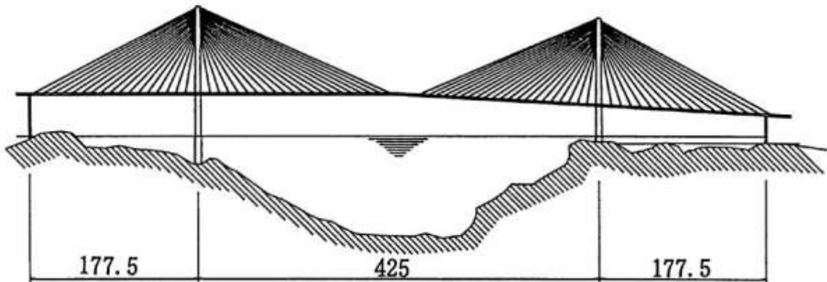
LSB20205,HELGELAND,
