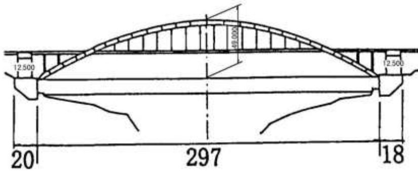
LSB30118,OHMISHIMA,大三島橋
