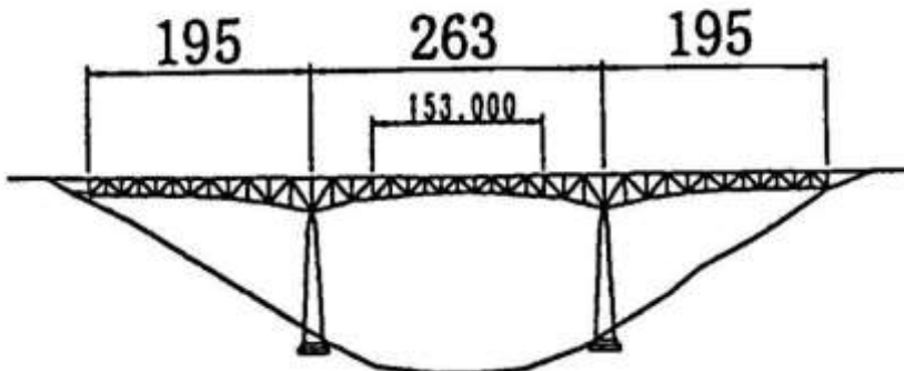
LSB40129,AUBURN-FORESTHILL,
