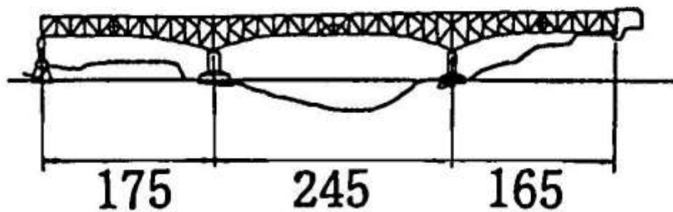
LSB40215, YOSHIMA, 与島橋
