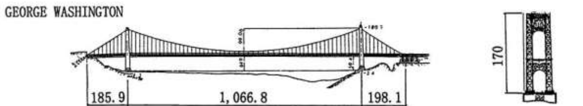
LSB10113, GEORGE WASHINGTON,
