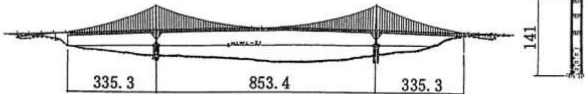
LSB10124, TACOMA NARROWS (NEW),
