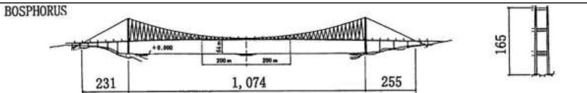
LSB10112, BOSPHORUS,
