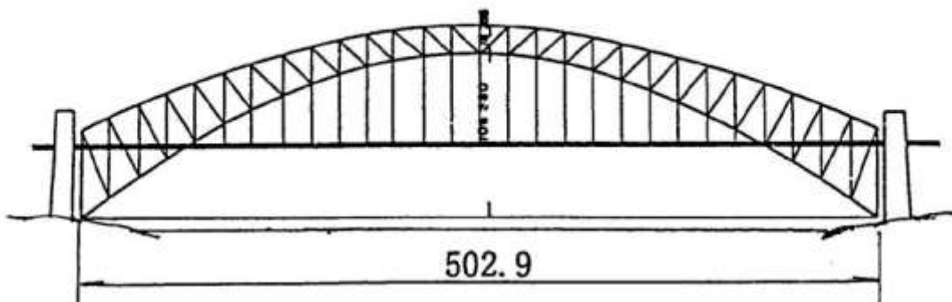
LSB30103,SYDNEY-HARBOUR,
