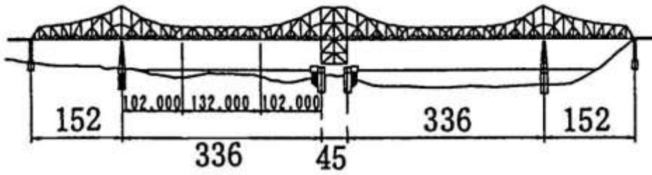
LSB40113,CARQUINEZ RAIT,
