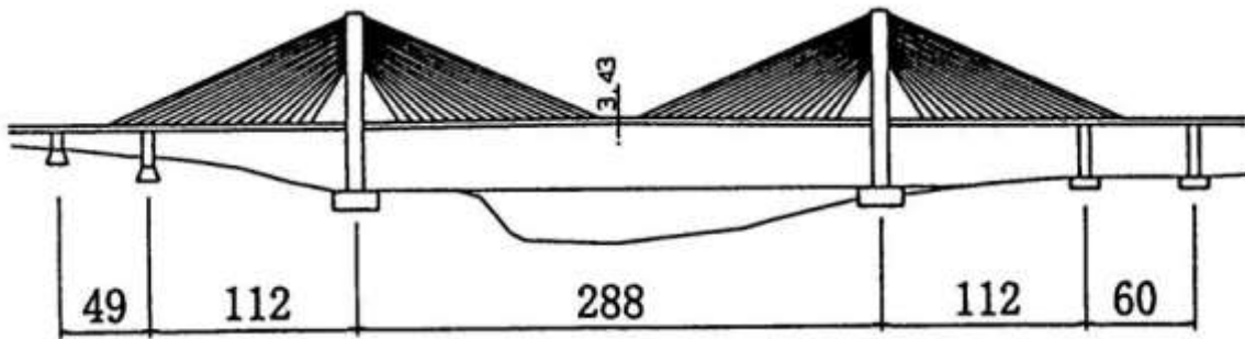
LSB20218,COATZACOALCOS-II,
