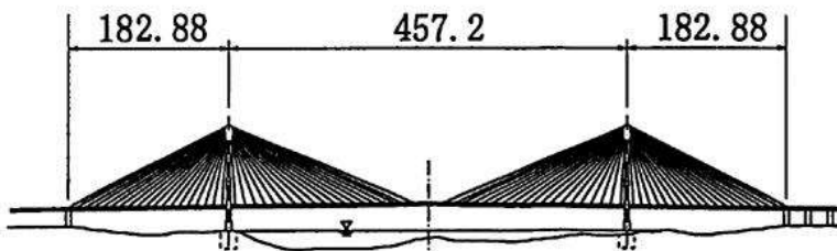
LSB20111,VIDYASAGAR-SETU (SECONDDHOOGHLY),
