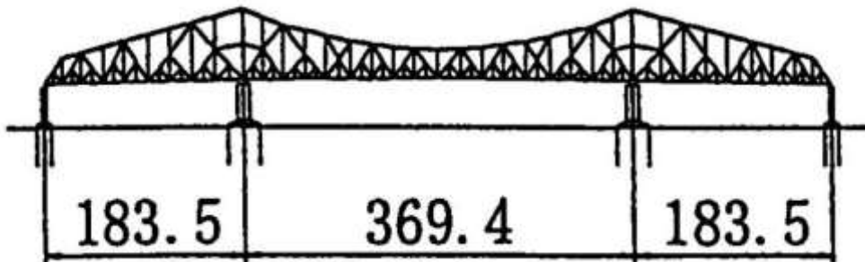
LSB40110,TAPPAN ZEE,
