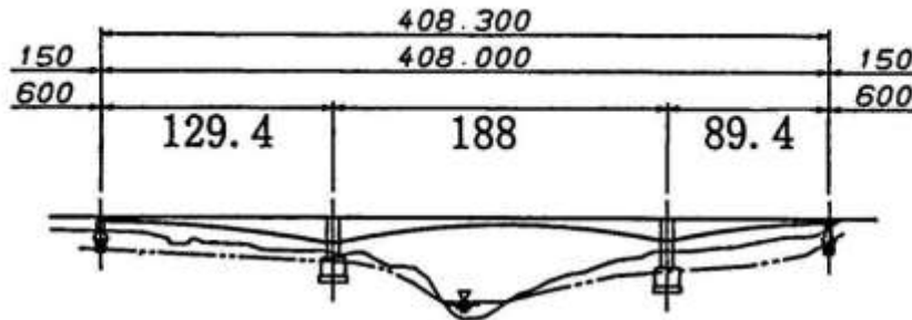
LSB50334,SHIN-HATCHIMANTAI,新八幡平橋,
