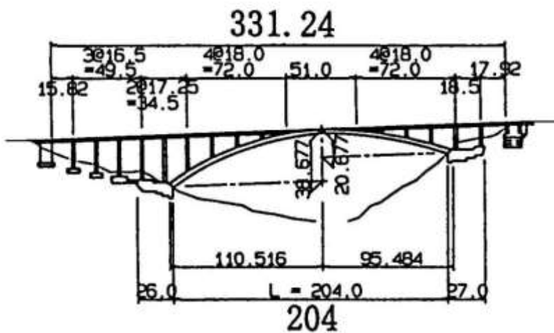
LSB30217, USAGAWA, 宇佐川橋
