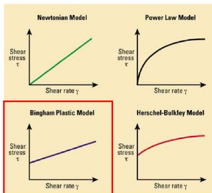
X-Y plots of rheological models.
